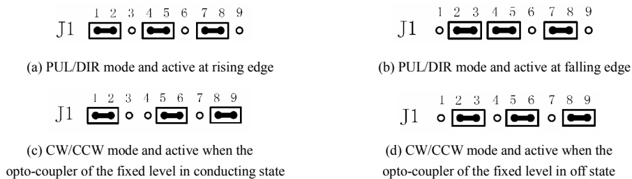
Figure 2: Control signal mode setting jumper
