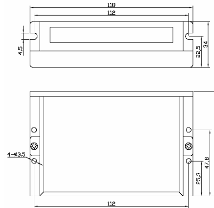
Figure 1: Mechanical specifications
